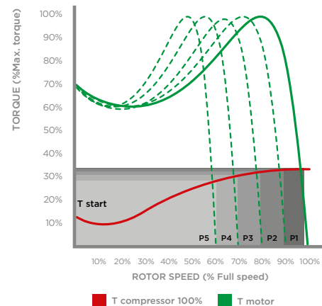
VSD CONTROL
