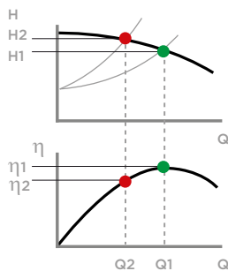
THROTTLING CONTROL
