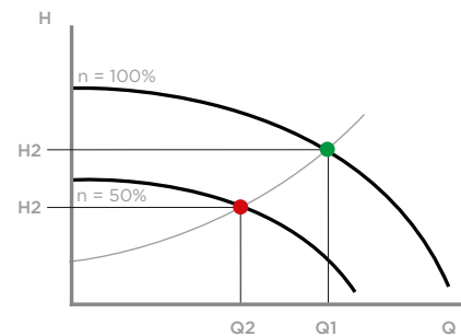
VSD CONTROL
